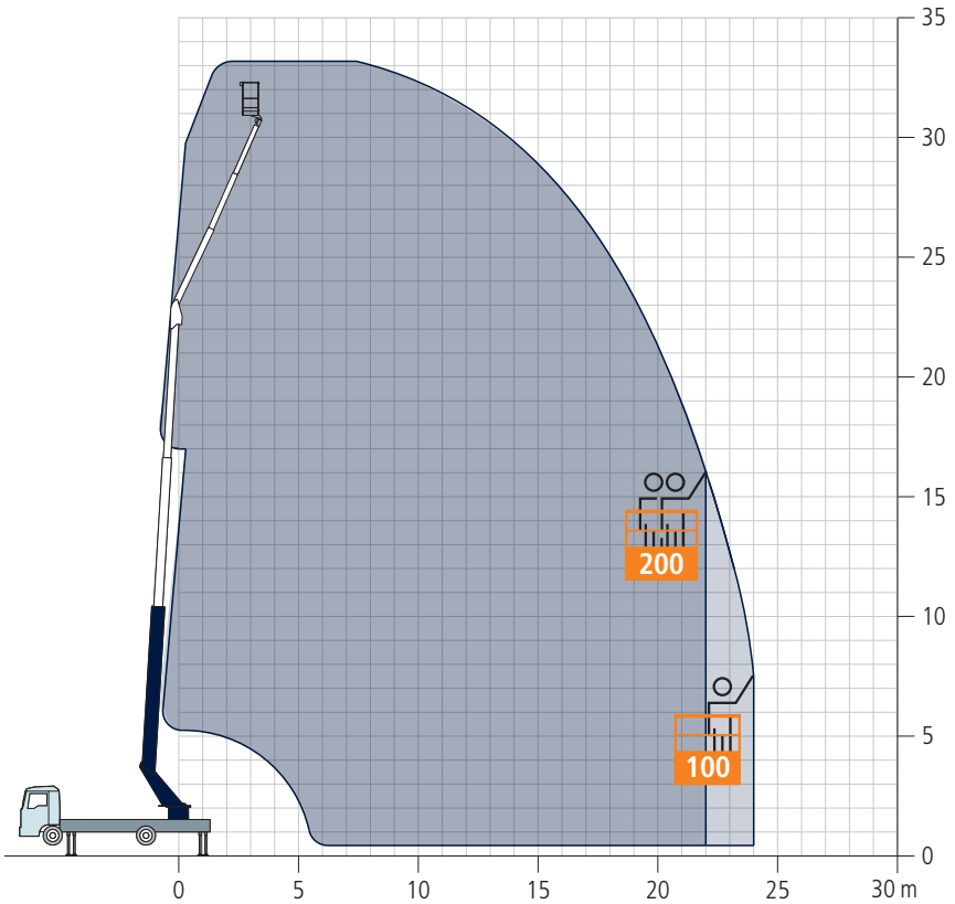
PK 250-D Ironing Basket, maximum load capacity of 200 kg
